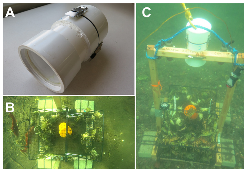
Fig. 3. Photographs depicting (A) a completed camera housing, (B) an example screen grab from a camera system deployment, and (C) the fully assembled camera system, deployed at sea.
