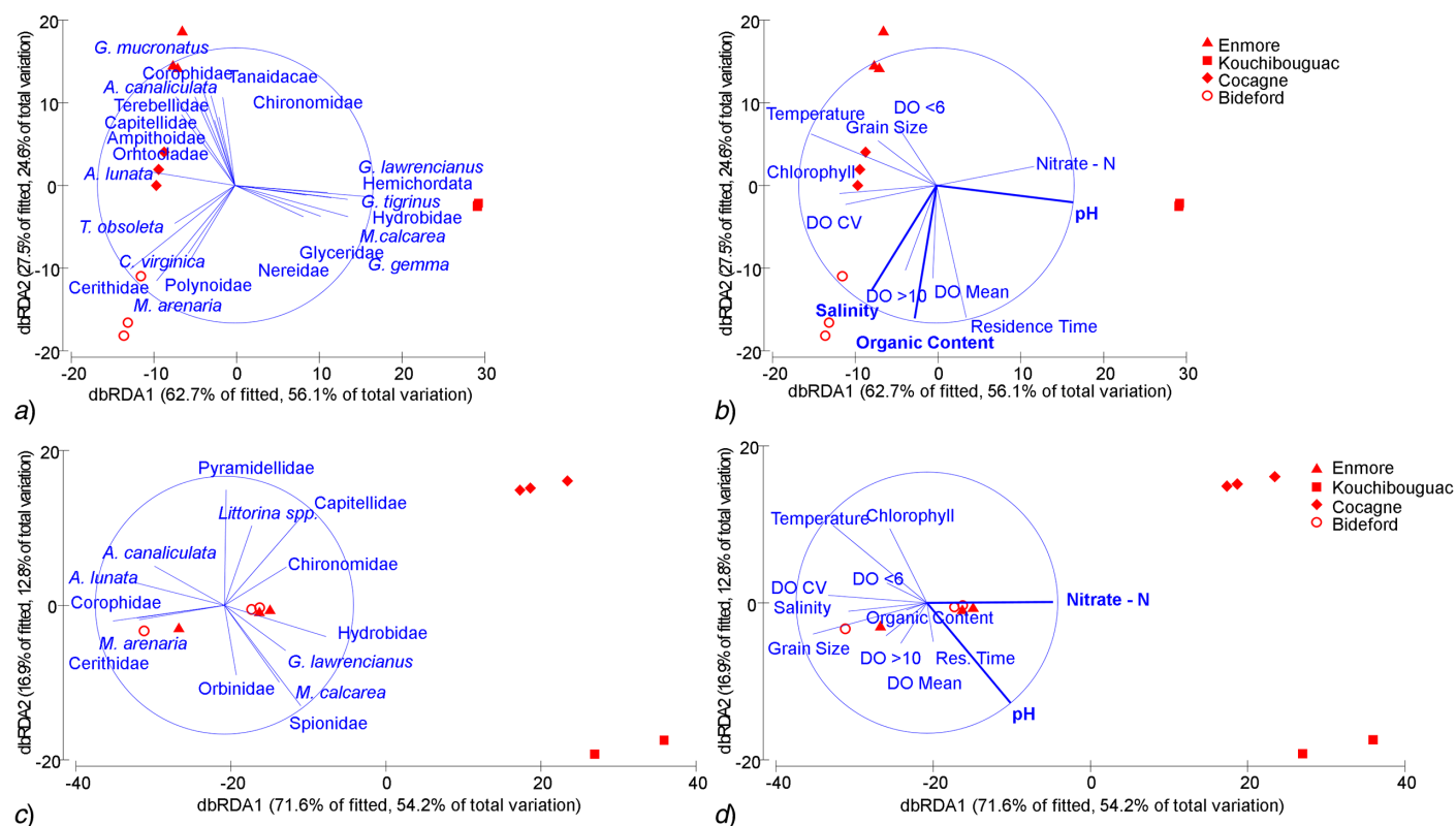
Fig. 4. Distance-based redundancy analysis (dbRDA) ordination plot of species (a, c) and environmental variables (b, d) of epifauna (a and b) and infauna (c and d) communities in Zostera marina . Vector length corresponds to a Pearson's correlation of r < 0.5 . Significant predictor variables from the distance-based linear models are bolded in the ordinations. Sites are represented by the symbols used in previous figures with samples representing the average abundance of a species between all samples per sampling time (month). DO, dissolved oxygen; CV, coefficient of variation.
