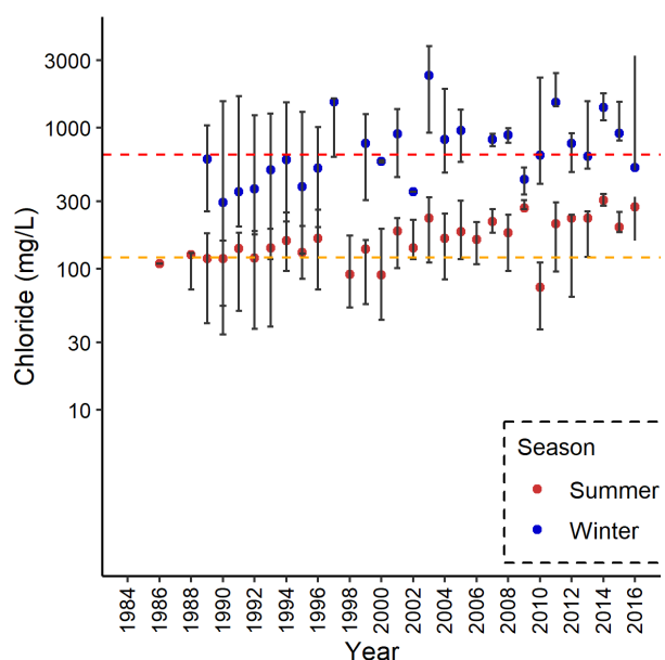
Fig. 1. Ontario Provincial Stream Water Quality Monitoring Network chloride data 1984–2016 for the Don River Pottery Road (06008501402) sampling station in Toronto, Canada (Site I in Fig. S1 ). Circles represent median chloride levels per year and season, and error bars indicate the 5th and 95th quantiles. Summer period includes the months of June, July, and August, while winter period includes January, February, and March. Data available sampled from 1986 to 2016 ( n = 395 ). The orange dashed line represents the Canadian government threshold for chronic chloride exposure (120 mg/L), the red dashed line represents the Canadian government threshold for acute chloride exposure (640 mg/L). Note the logarithmic scale for chloride concentrations.
