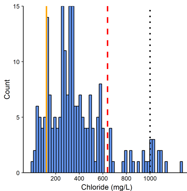
Fig. 5. Histogram of summer chloride concentrations found at sites in the current study ( n = 214 ). Yellow solid line indicates the federal chronic threshold of 120 mg/L Cl. Red dashed line indicates the federal acute limit of 640 mg/L Cl. Black dashed line indicates 1000 mg/L Cl.
